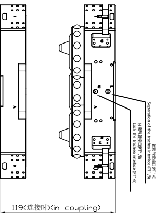
119(连接时)(in coupling)
